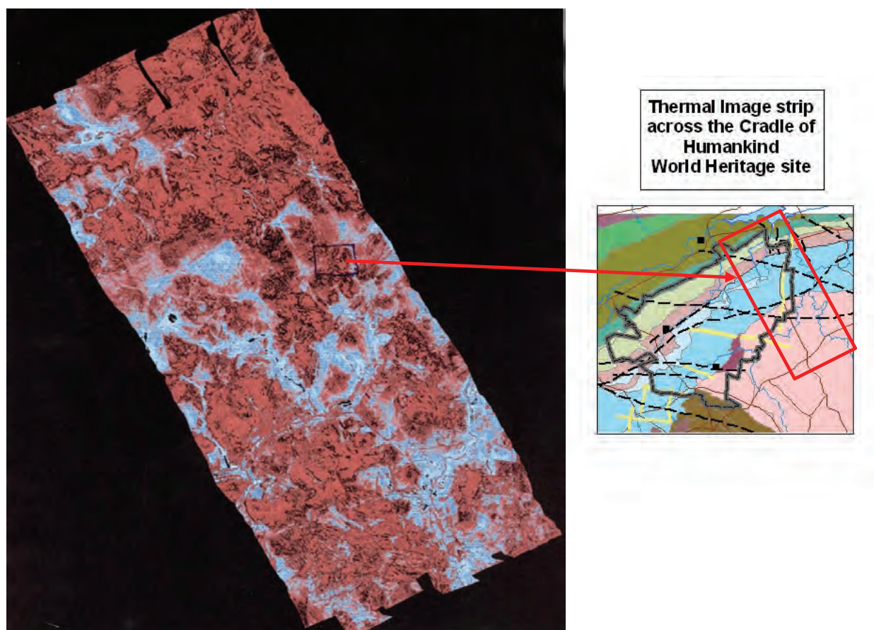
Figure 6.4: Colour table enhanced thermal image of the central Cradle area showing the cold wet surface areas in blue, marking the saturated compartments, and the bounding linear structure zones (Adapted from image taken by Anglo American Geophysical Services (Jamison, 2001)).
